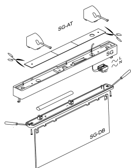
Montaje paralelo a pared Parallel to the wall
