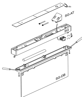
Montaje perpendicular a pared Perpendicular to the wall
