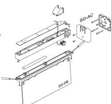
Montaje perpendicular a pared Perpendicular to the wall
