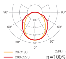
Maintained / Non-maintained multiled
